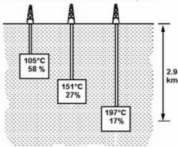
Helium retention in Jemez Caldera, NM
